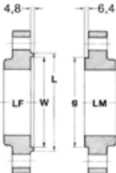
INCAMERATURA SEMPLICE LARGA LARGE MALE AND FEMALE
