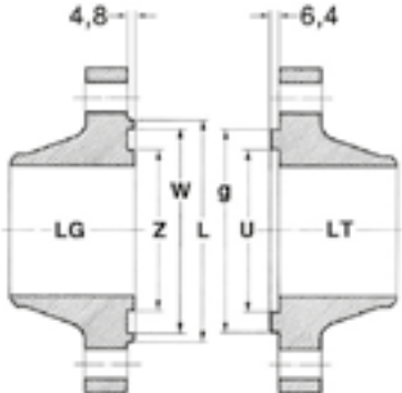
INCAMERATURA DOPPIA LARGA LARGE TONGUE AND GROOVE
